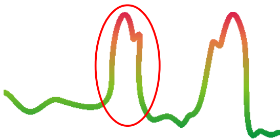
Figure 7.7: Signature of a non-ferromagnetic metal target
