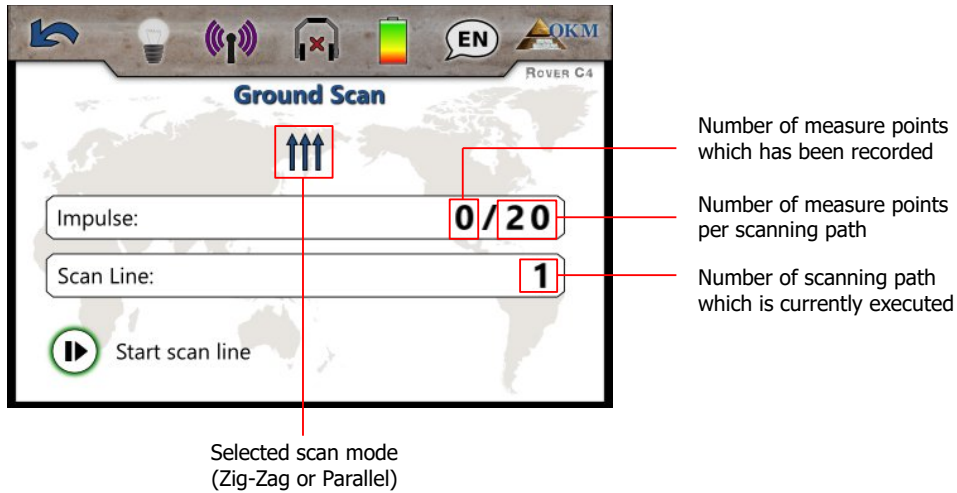
Figure 7.2: Display representation in operating mode "Ground Scan"
