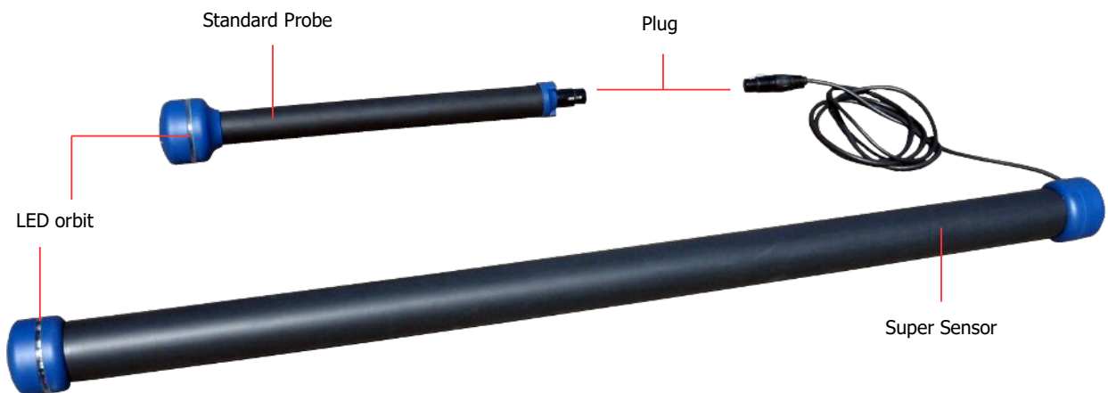
Figure 5.3: Control elements of the Probes
